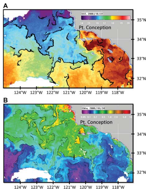
Fig. 1. Examples of detected fronts, shown as black contours on top of a SST image ( A , MODIS Aqua, 22 October 2008) and a chlorophyll- a (mg m -3 ) image ( B , MERIS, 24 October 2008). White areas are clouds. Black vertically spaced dots across a front near the center show the locations of CTD-UVP5/Bongo stations between cycles 5 and 6 of the A-Front study.
