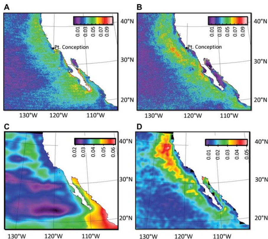
Fig. 3. Overall mean FF for SST ( A , 1981–2009) and Chl ( B , 1997–2010). Variance of the sea level height anomaly ( \text{m}^2 ) separated into the large-scale component ( C ) and mesoscale ( D ) component.
