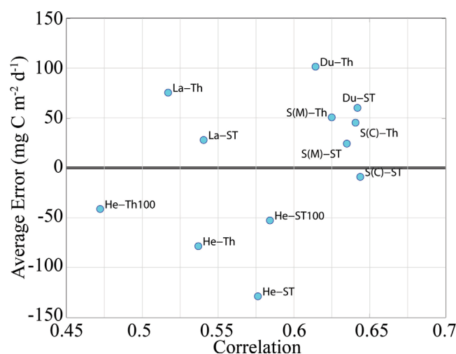
Figure 4. Model average error and correlation for different satellite algorithms when compared to ^{234}\text{Th} (Th) or sediment trap (ST) data. Models are Laws 2011 (La), Dunne 2005. (Du), Henson 2011 (He), Siegel 2011, with the fraction of microphytoplankton determined by microscopy (S(M)), and Siegel 2011, with the fraction of microphytoplankton determined by size-fractionated Chl a (S(C)). All models are compared to export normalized to the depth of EZ except for He-Th100 and He-ST100, which were normalized to 100 m, since the Henson 2011 algorithm was specifically designed for that depth.
